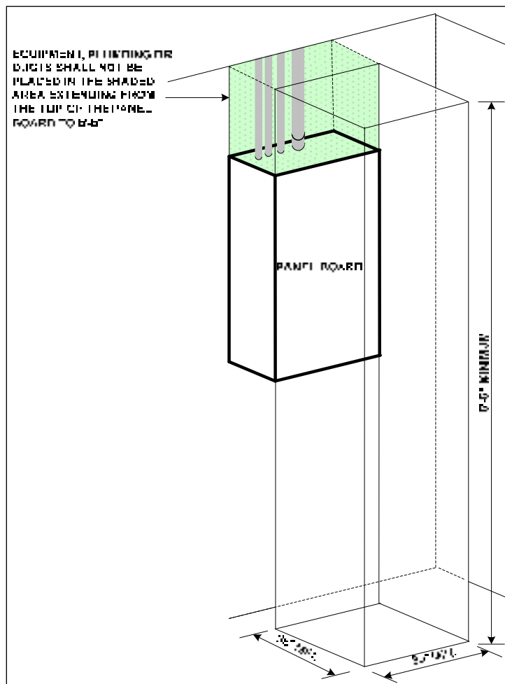
FIGURE 14: Panel Board
