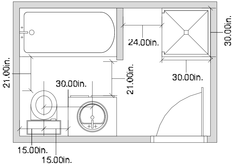
FIGURE 13: Bath Group Fixture Clearances
