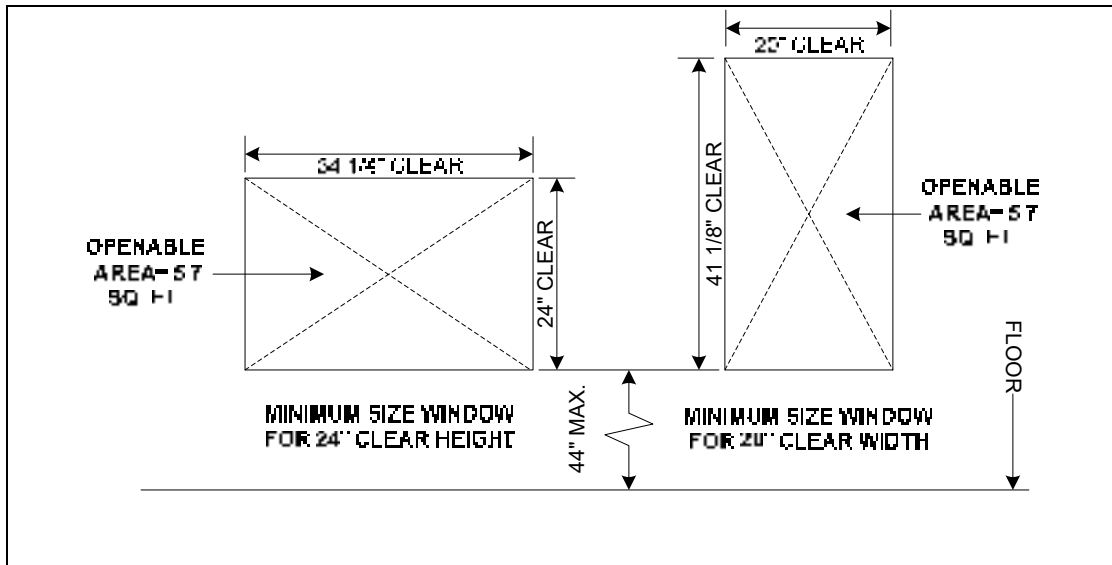
Minimum width and height requirements for an egress window opening to meet 5.7 sq.ft.
