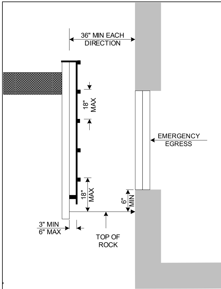
FIGURE 2: Typical Window Well Requirements
