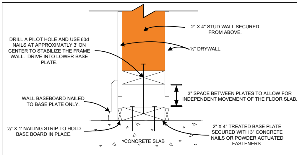
FIGURE 8: Non-bearing Slab on Grade Wall Framing
